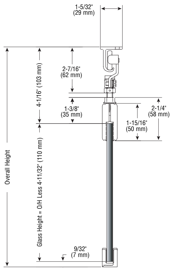
Single Track Installation
